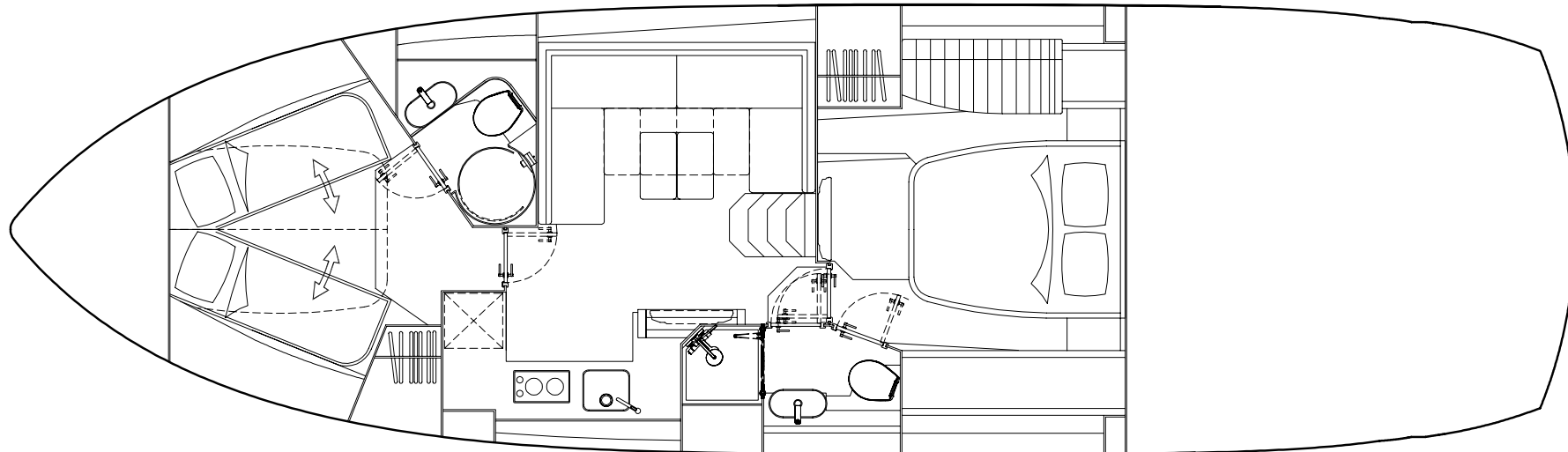
Lower deck
