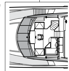
Raised wheelhouse
